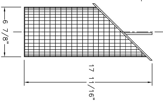
BASKET DETAIL
