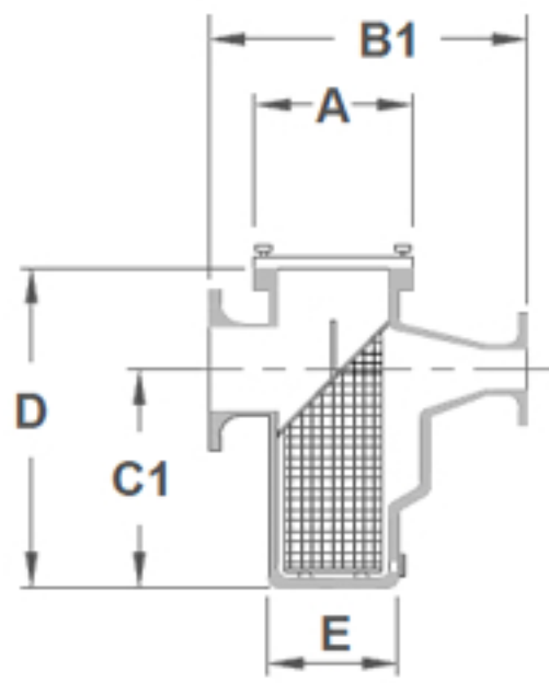
CONCENTRIC REDUCER
